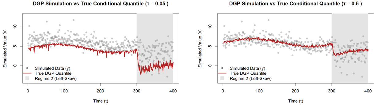
(a) DGP and Theoretical Quantiles ( \tau = 0.05 )
