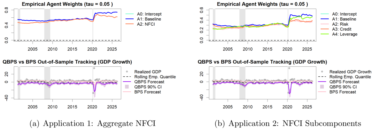
Figure 6: QBPS: DYNAMIC WEIGHTING AND TAIL FORECASTS
