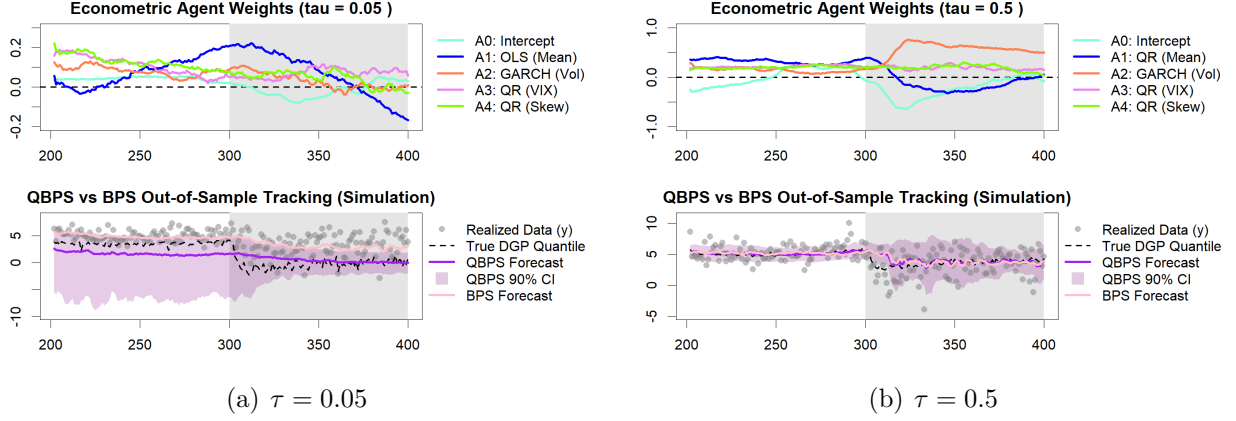
Figure 3: QBPS: DYNAMIC WEIGHTING AND TAIL FORECASTS (PARAMETRIC AGENTS)
