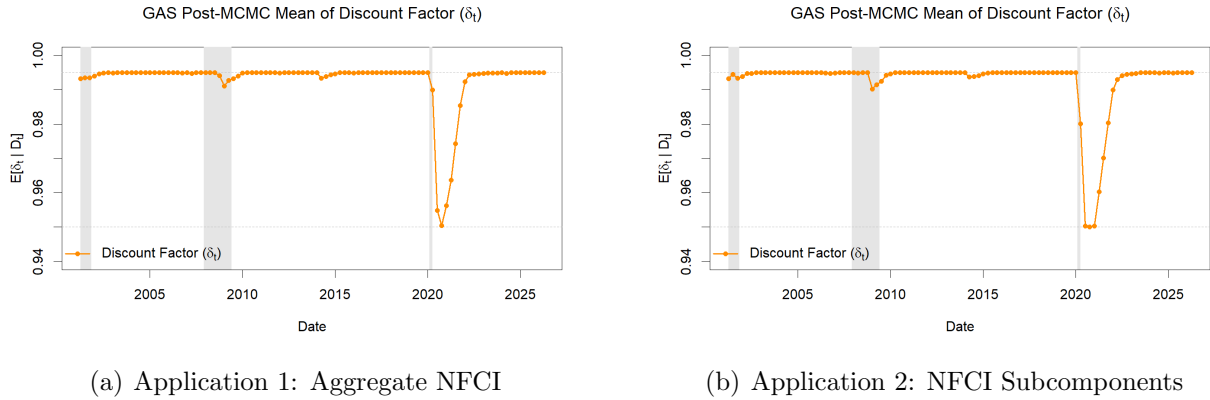
Figure 7: SCORE-DRIVEN ADAPTATION VIA DYNAMIC DISCOUNTING
