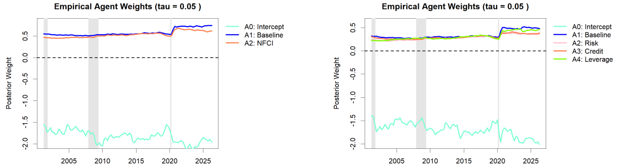
(a) Application 1: Aggregate NFCI
