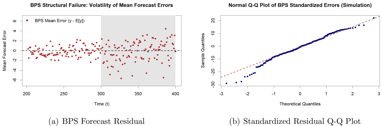
Figure 2: GAUSSIAN BENCHMARK (BPS) MEAN FORECAST RESIDUALS
