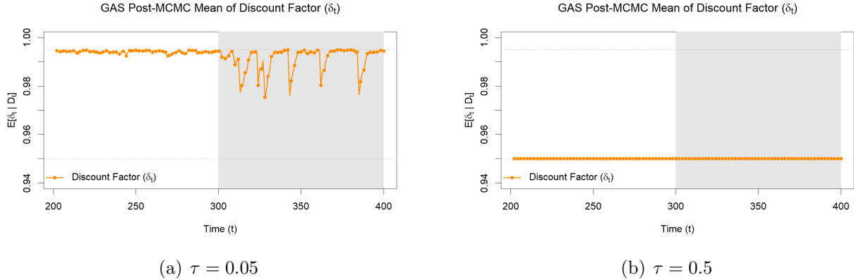
Figure 4: SCORE-DRIVEN DYNAMIC DISCOUNTING (PARAMETRIC AGENTS)
