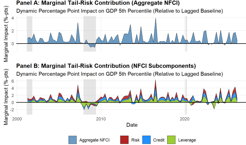
Figure 8: DYNAMIC GROWTH-AT-RISK (GaR) MARGINAL ATTRIBUTION
